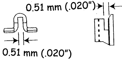
Fig. 3a bracket specifications
